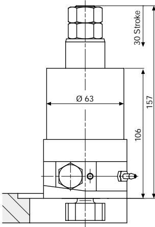
Tie rod retracted Swivelling angle 0°
