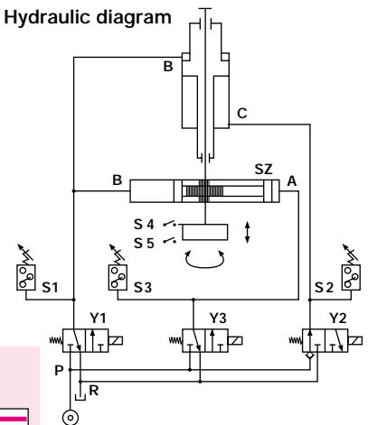
Hydraulic diagram
