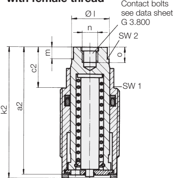
Version with female thread
