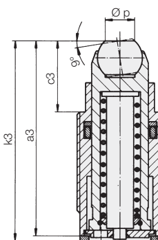
Version with swivel contact bolt
