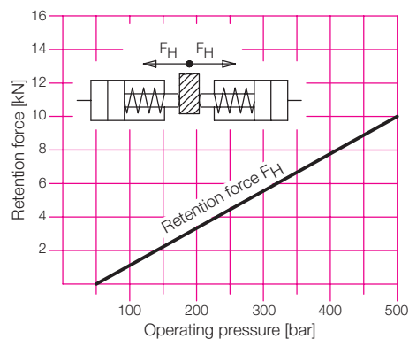
Retention force for "floating clamping"
