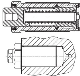
Threaded-body cylinder with locking piston (page 2)
