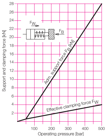
Effective clamping force and admissible load
