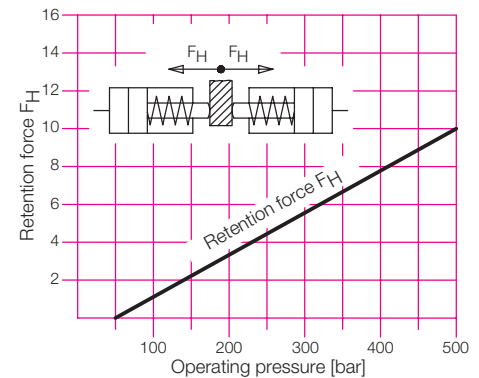
Retention force for "floating clamping"
