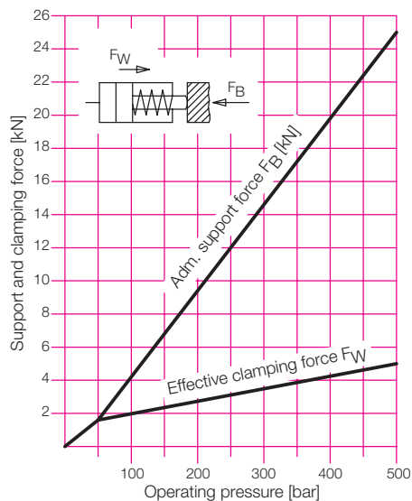
Effective clamping force and admissible load
