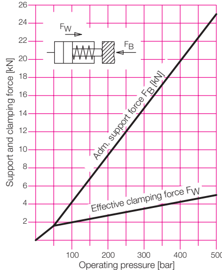
Effective clamping force and admissible load
