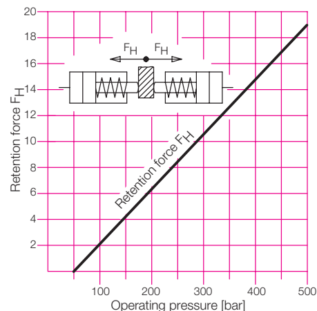
Retention force for "floating clamping"
