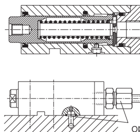
Block cylinder with locking piston (page 3)
