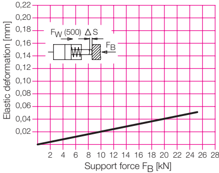
Elastic deformation as a function of the support force of the piston at an operating pressure of 500 bar
