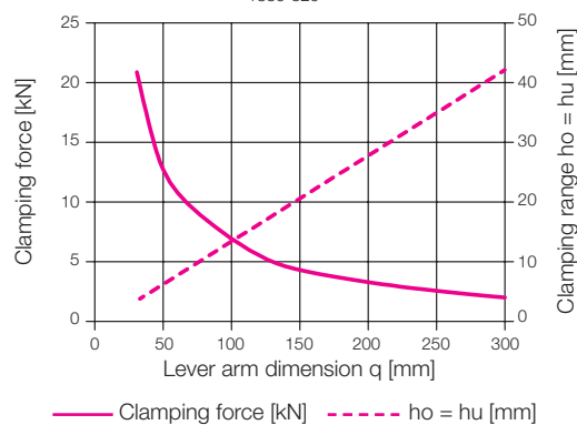
Clamping force/clamping stroke for longer special clamping levers 1830-330
