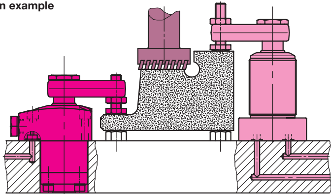
Flange with O-ring sealing for manifold mounting
